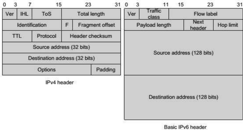
Figure 1-1 format comparison of IPv4 message header and IPv6 basic message header
