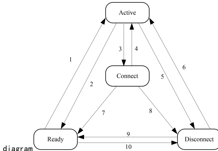
Command switch state transition
