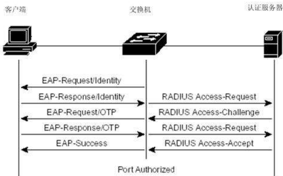
Re authenticated protocol
