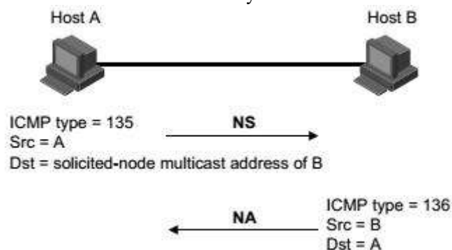
Figure 1-3 schematic diagram of address resolution
