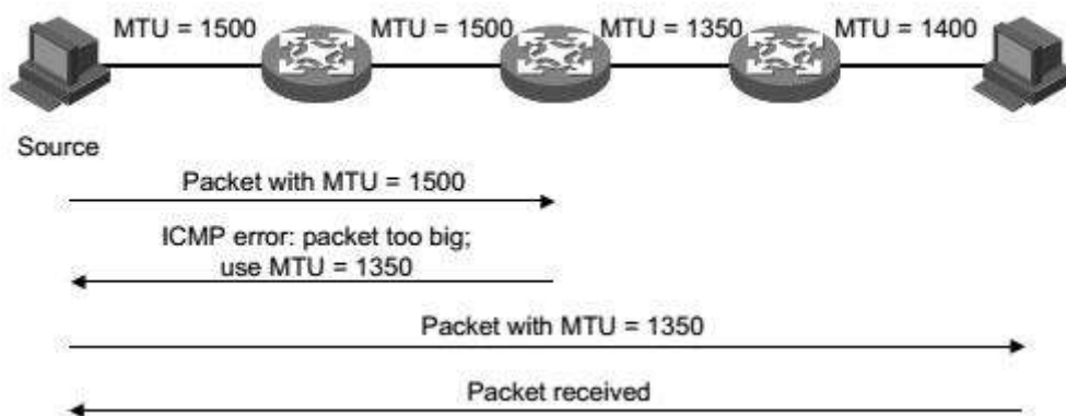
Figure 1-5 pmtu discovery process
